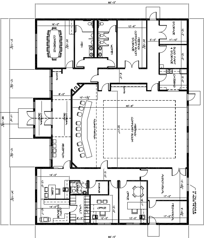
FLOOR PLAN SCALE 1/8"=1'-0"
